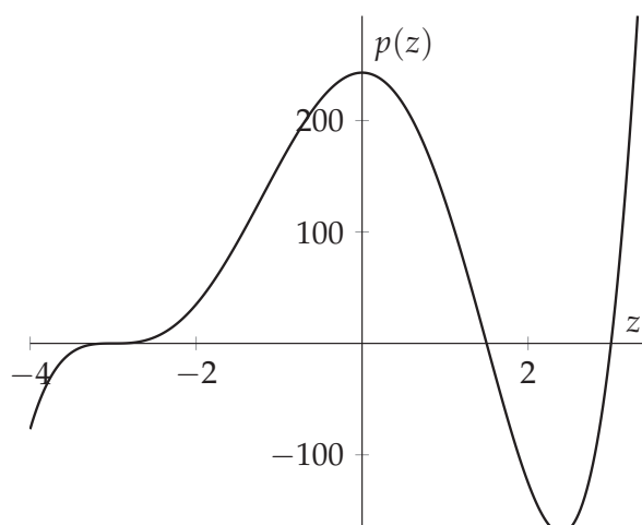
Figur 5.3: Grafen for polynomiumsfunctioen p : \mathbb{R} \rightarrow \mathbb{R} , hvor p(z) = 2z^5 + 9z^4 - 18z^3 - 108z^2 + 243 .
